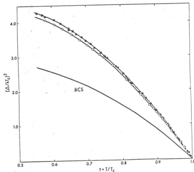
FIG. 2. Squared reduced energy gap (at the gap edge) of Pb as a function of reduced temperature. Black dots and squares, P=0 ; open circles, P=2730 bar.
